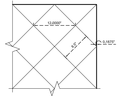
Corner Detail Scale: 3/4" = 1'-0"
